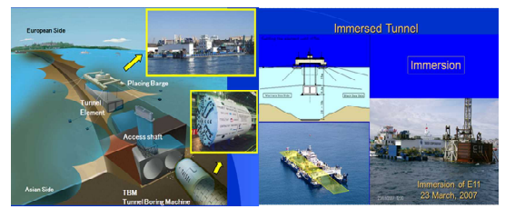
【 Turkey 】 Railway Bosphorus Tube Crossing, Tunnels and stations (2014)
